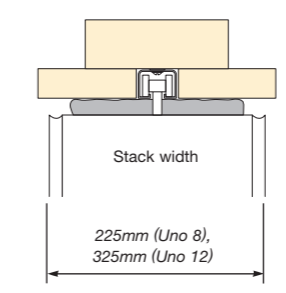
Track with acoustic seal
