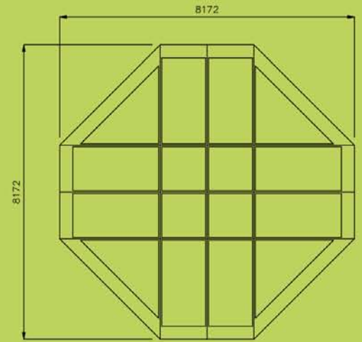
PLAN VIEW SFP062
