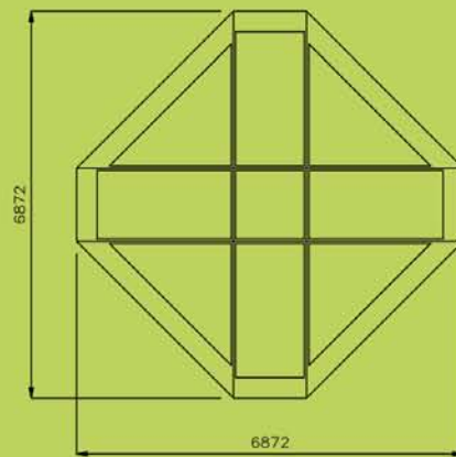
PLAN VIEW SFP061
