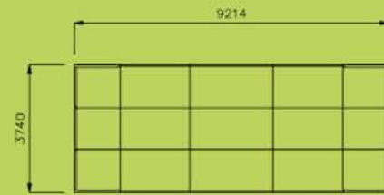
PLAN VIEW SHP123
