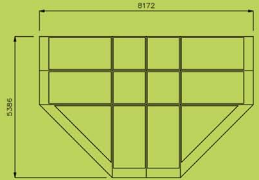
PLAN VIEW SHP062
