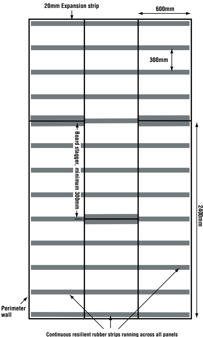
Typical floor layout
