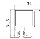
PF17.09 Interlock section
