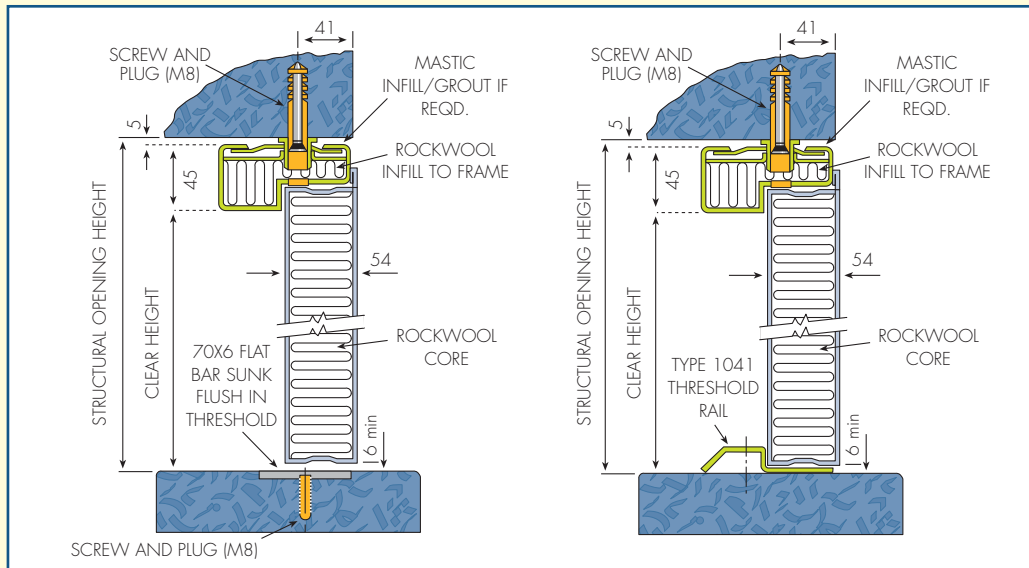
End section flat bar cill
