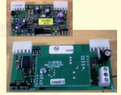
Loop Card and Radio Receiver Card
