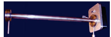
Fig. 2 SS2000 Laser system Tunable diode laser system uses NIR light at a specific wavelength to determine moisture content.
